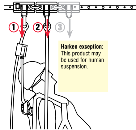
Pinstop car allows movement of cars along track. Open to move; close to lock in place.
